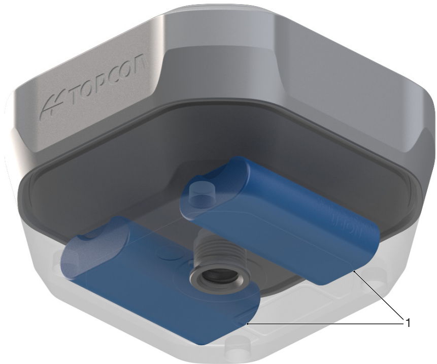
1 Internal battery pack (two batteries – bottom view)
