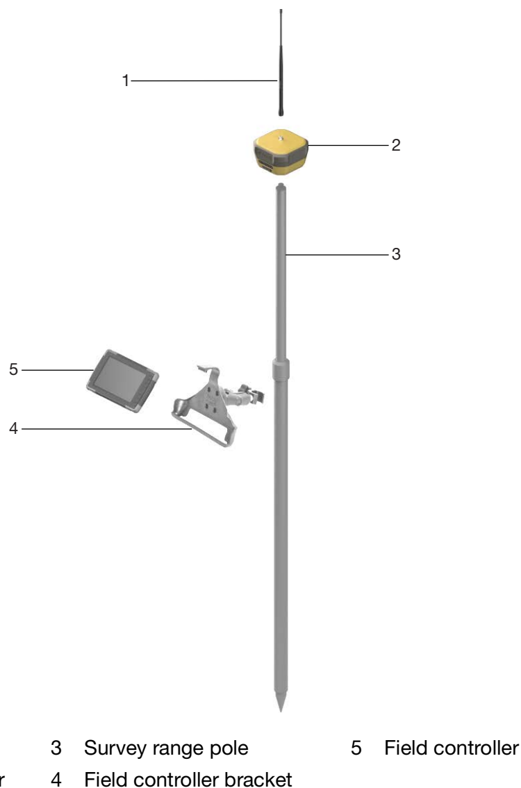
Figure 3-6: General RTK Rover Setup
