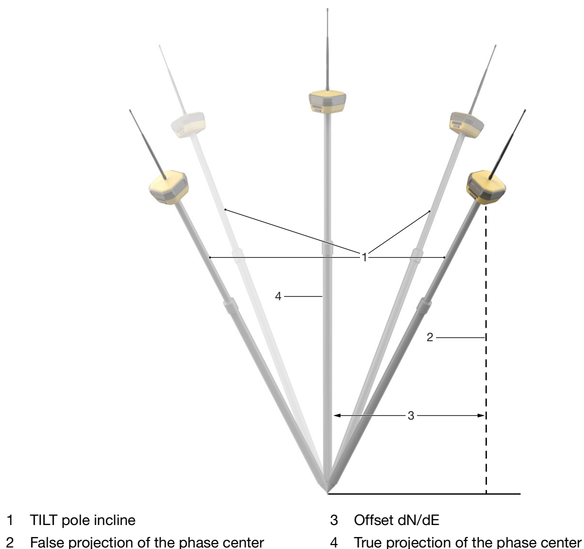
Figure 3-7: TILT Alignment Positions
