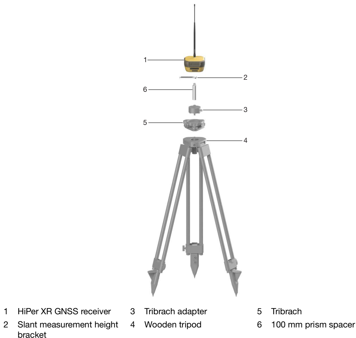
Figure 3-1: General Static Setup
