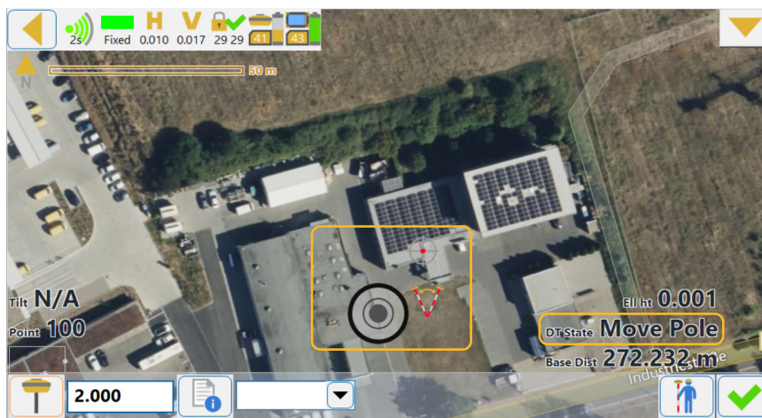
Figure 3-13: TILT Move Pole State
